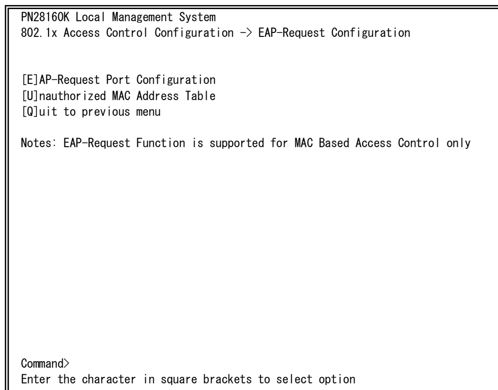
図4-7-25-14 EAP-Request Configuration
