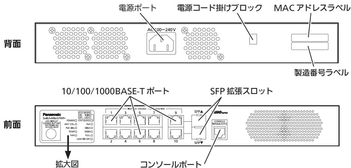
図1-1 Switch-M8eGPWR+
