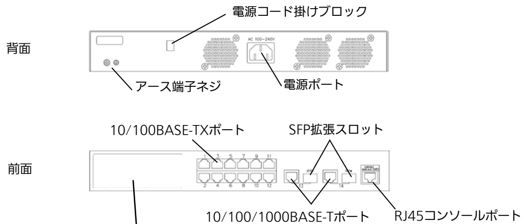
図1-1 Switch-M12PWR
