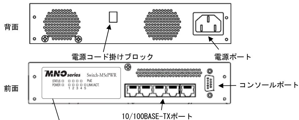
図1-1 Switch-M5ePWR
