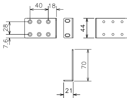
Mounting bracket (for 19-inch rack)
