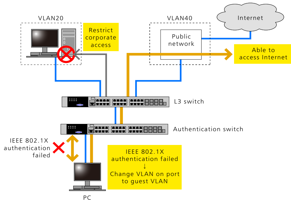
Figure 70-4 Connection through guest VLAN
