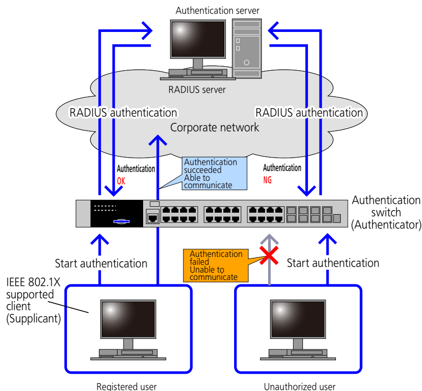
Figure 70-2 IEEE 802.1X overview
