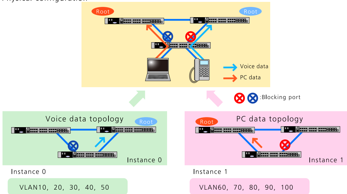
Figure 76-3 MSTP overview
