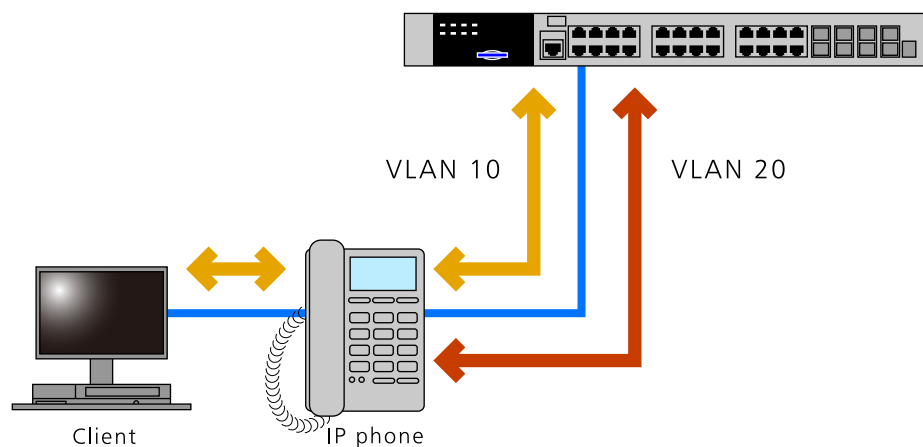
Figure 36-1 Voice VLAN overview
