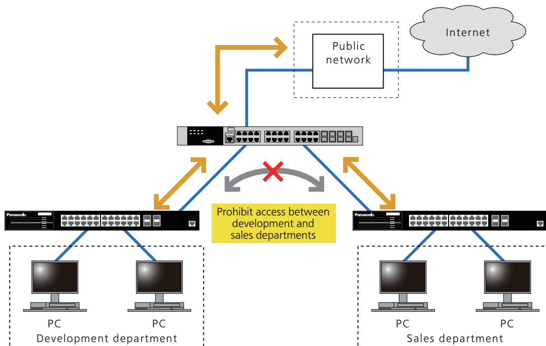
Figure 42-1 Access Control overview
