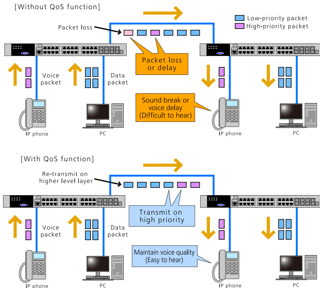
Figure 43-1 QoS overview
