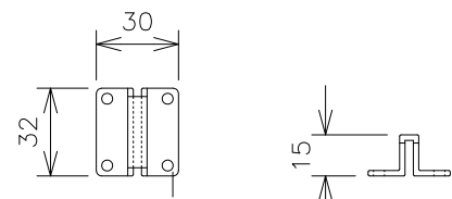
Connecting bracket
