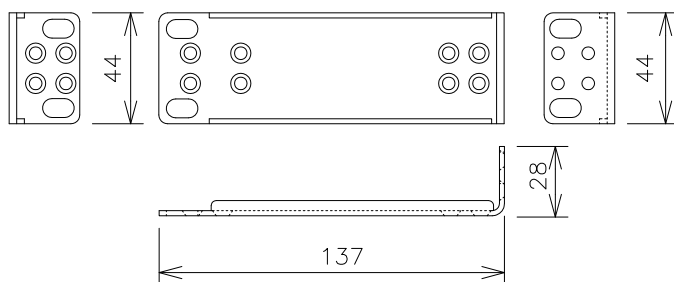
Mounting bracket (for 19-inch rack)
