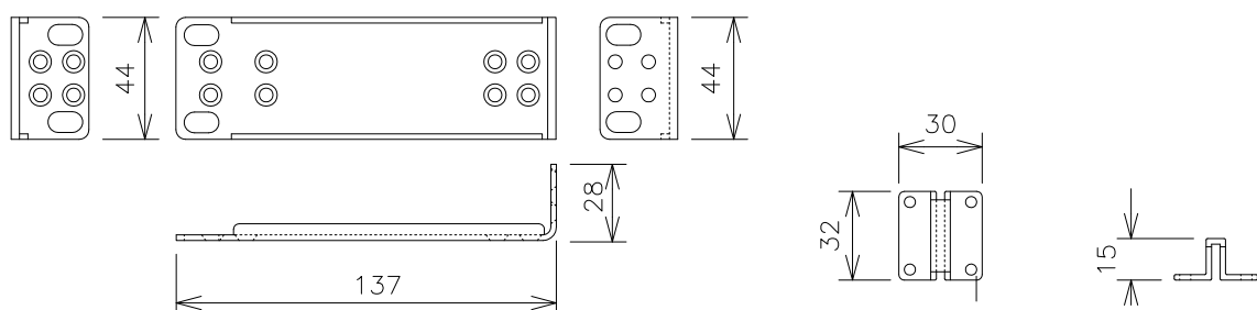
Mounting bracket (for 19-inch rack)
