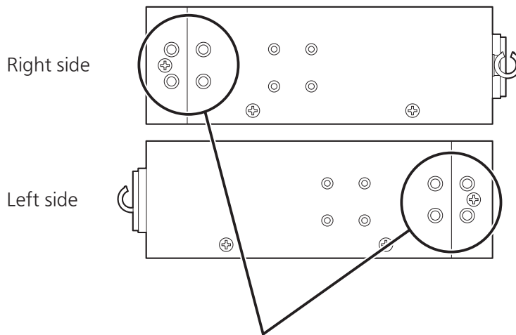
Screw holes for fixing the 19-inch rack mount brackets
