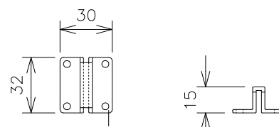
Connecting bracket
