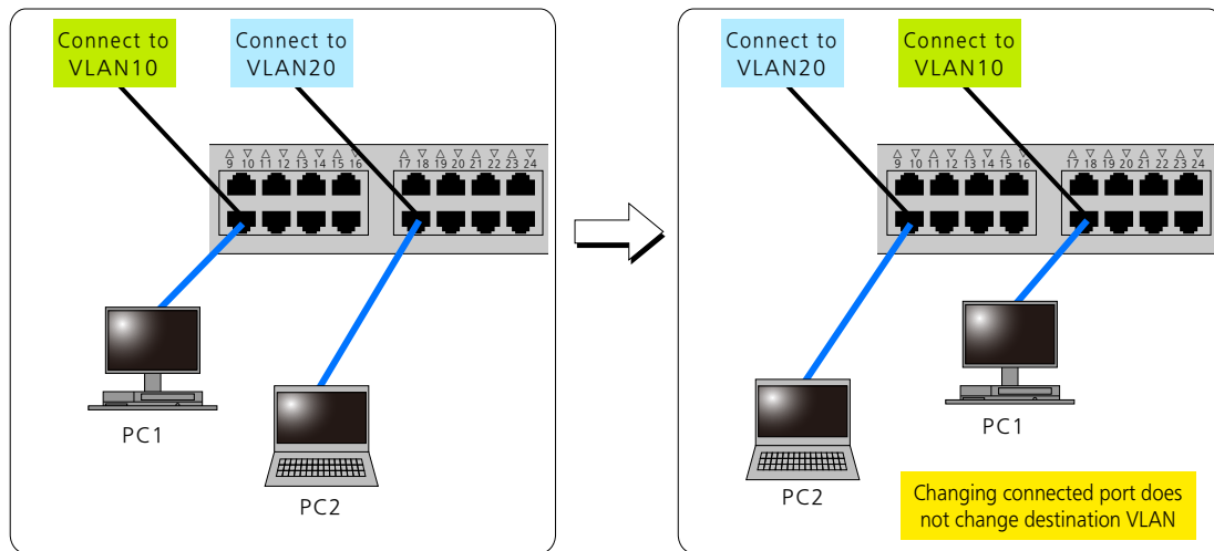
Figure 66-5 Dynamic VLAN
