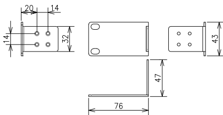
Mounting bracket (for 19-inch rack)
