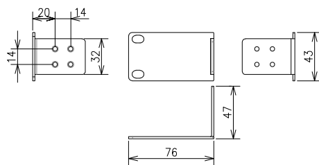
Mounting bracket (for 19-inch rack)
