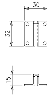
Connecting bracket
