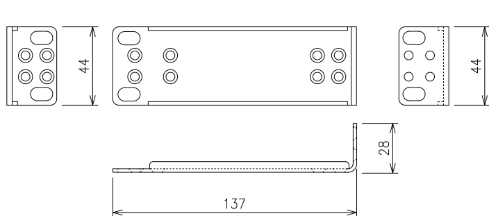
Mounting bracket (for 19-inch rack)
