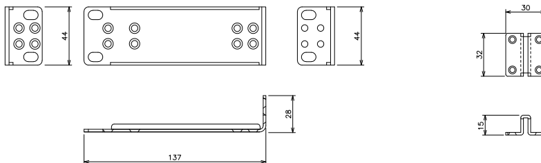
Mounting bracket(for 19-inch rack)
