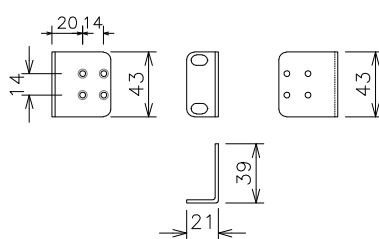
Mounting bracket(for 19-inch rack)
