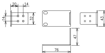
Mounting bracket (for 19-inch rack)
