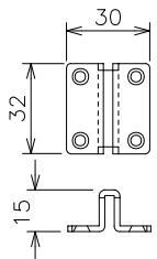
Connecting bracket
